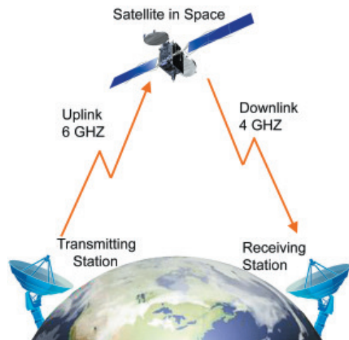
Fig. 8.14 : Satellite link
