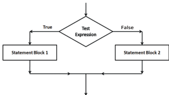
Fig 7.2: Flowchart of if-else
